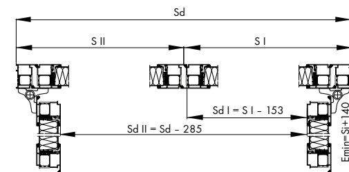
Fig. 80. Installation in the opening - horizontal section - double-leaf door - the MB86 ST system.
