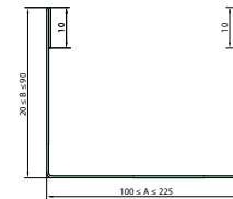
Fig. 82. Fascia panel type D
