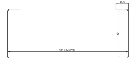
Fig. 84. Fascia panel type F
