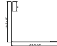
Fig. 80. Fascia panel type B
