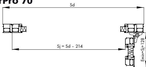
Fig. 74. Installation in the opening - horizontal section - single-leaf door - the MB70 system.
