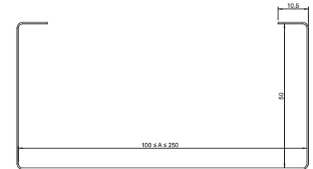
Fig. 85. Fascia panel type G
