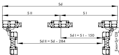
Fig. 75. Installation in the opening - horizontal section - double-leaf door - the MB70 system.
