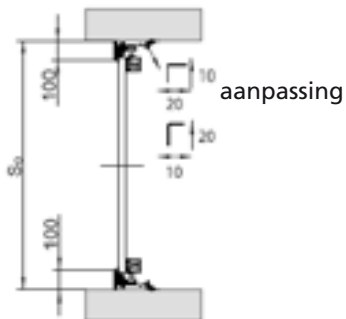
Horizontale doorsnede, montage IN de opening
