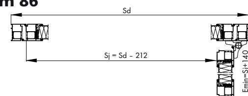
Fig. 79. Installation in the opening - horizontal section - single-leaf door - the MB86 ST system.
