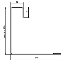
Fig. 79. Fascia panel type A
