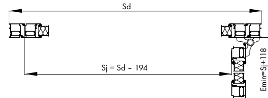
Fig. 71. Installation in the opening - horizontal section - single-leaf door - the MB60E system.
