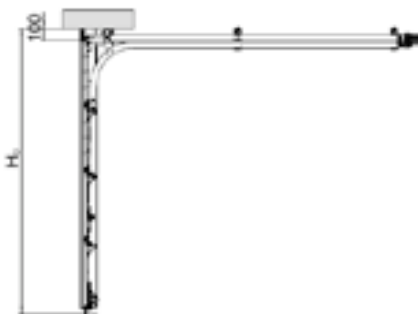
Verticale doorsnede, montage IN de opening
