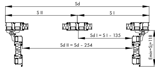
Fig. 72. Installation in the opening - horizontal section - double-leaf door - the MB60E system.
